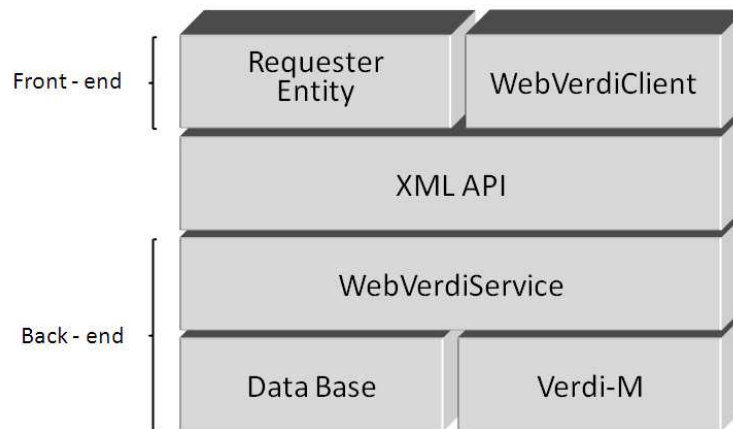
Fig. 1. Components of WebVerdi-M
