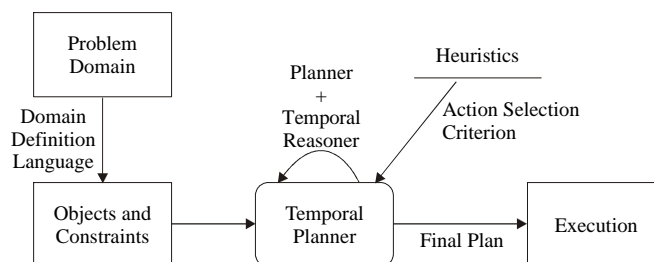
Figure 2: Temporal planning approach
