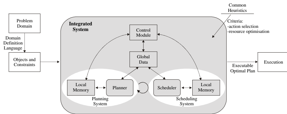
Figure 3: Structure of the integrated system of planning and scheduling
