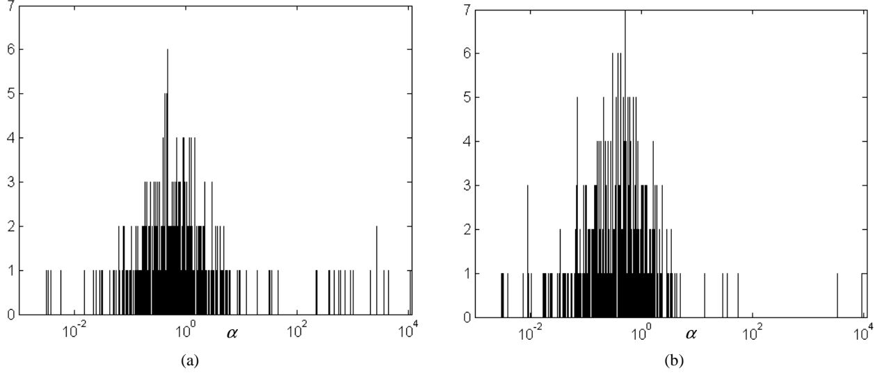
Fig. 1. Example of the distributions of the ratio -\frac{\Delta_{ij}^0}{\Delta_{ij}^1} evaluated on S_{10} (a) and S_{01} (b) .
