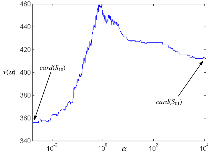
Fig. 2. The trend of v(\alpha)=F_{10}(\alpha)+F_{01}(\alpha) obtained by the two distributions shown in fig. 1. The points in which the combination reduces to one of the dichotomizers (see text) are shown.
