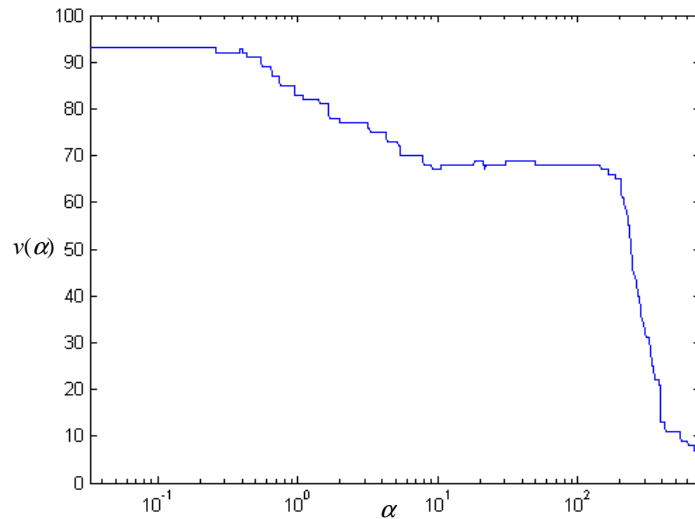
Fig. 4. The trend of \nu(\alpha)=F_{01}(\alpha)+F_{10}(\alpha) for the linear combination of an SL with an M4.
