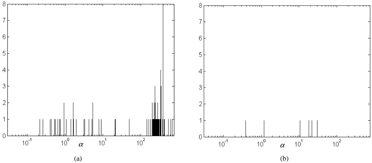
Fig. 3. The distributions of the ratio -\frac{\Delta_{ij}^0}{\Delta_{ij}^1} evaluated on S_{10} (a) and S_{01} (b) for the linear combination of an SL with an M4.
