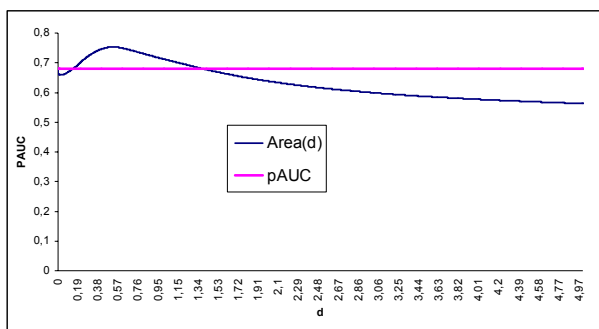
Figure 6. Oscillating area for increasing values of d gives two different d where \text{Area}(d) = \text{pAUC} .
