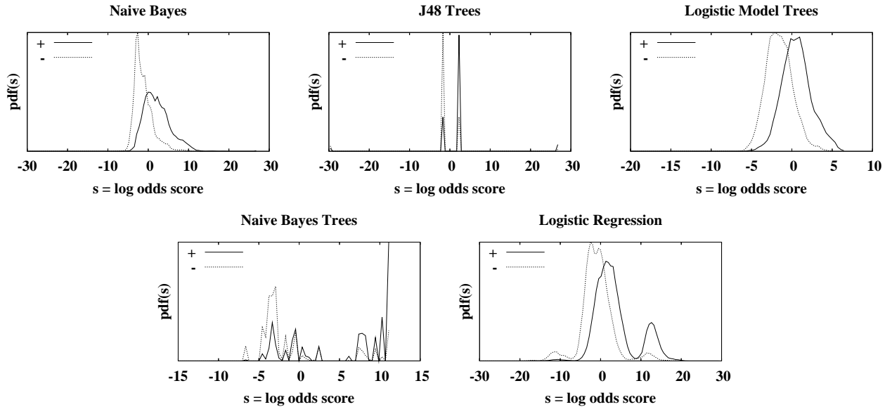
Figure 8. Score distributions of 5 Machine Learning methods on the Covertype data set.
