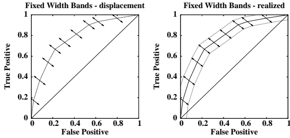
Figure 2. Displacing curve to generate FWB confidence bands.
