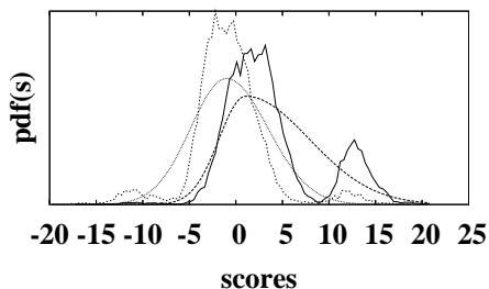
Figure 9. Sample logistic regression score distribution with r = 250000 . These distributions are clearly not unimodal.
