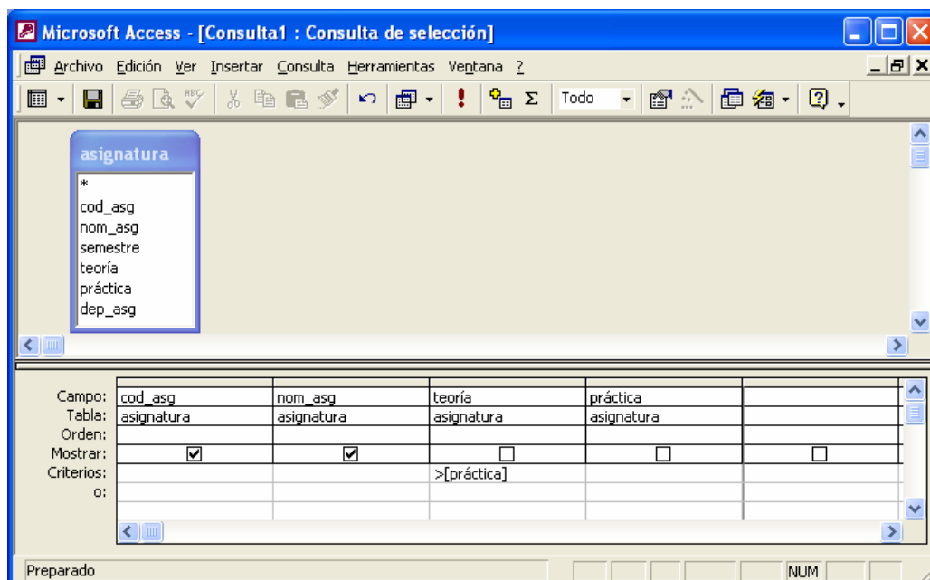
Figure 14: Example for the construction of a condition with references to other attributes.
