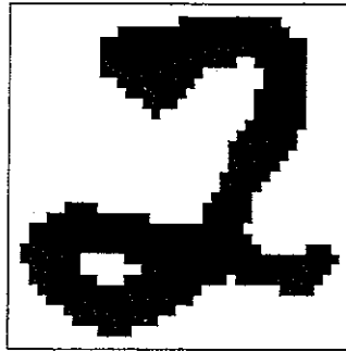
Fig. 1. Handwritten digit 2
