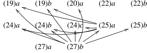
Figure 5: Variant-preserving dependency graph for Diffie-Hellman
