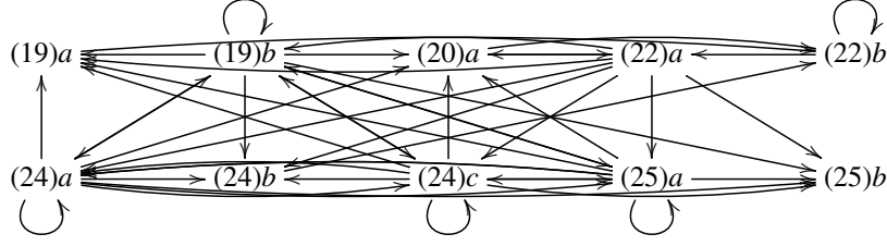
Figure 3: Dependency graph of Abelian group
