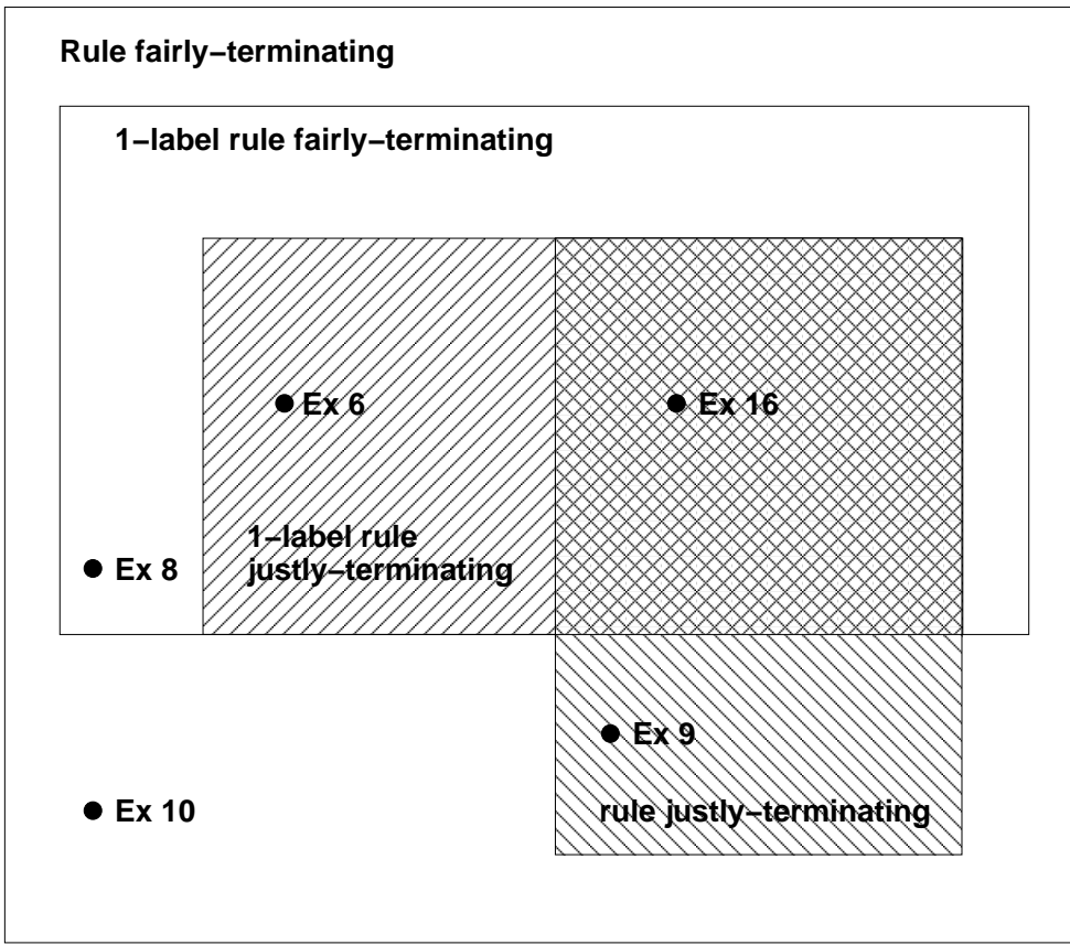
Fig. 1. Comparing Just/fair-termination properties
