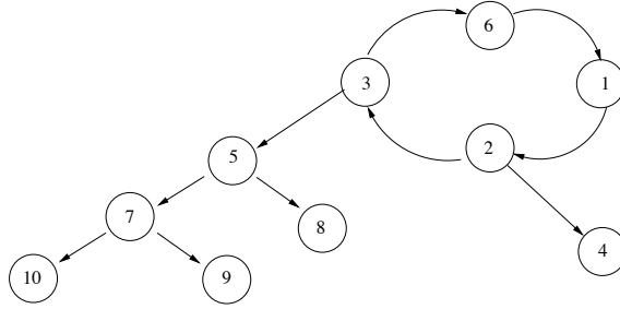
Fig. 5. Dependency graph for the transformed \mathcal{R}_{SplitD}
